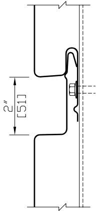
HORIZONTAL JOINT DETAIL
