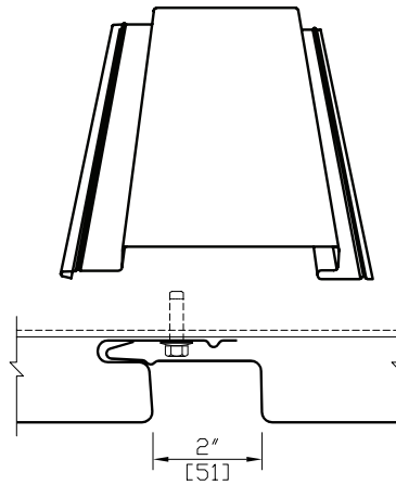
VERTICAL JOINT DETAIL
